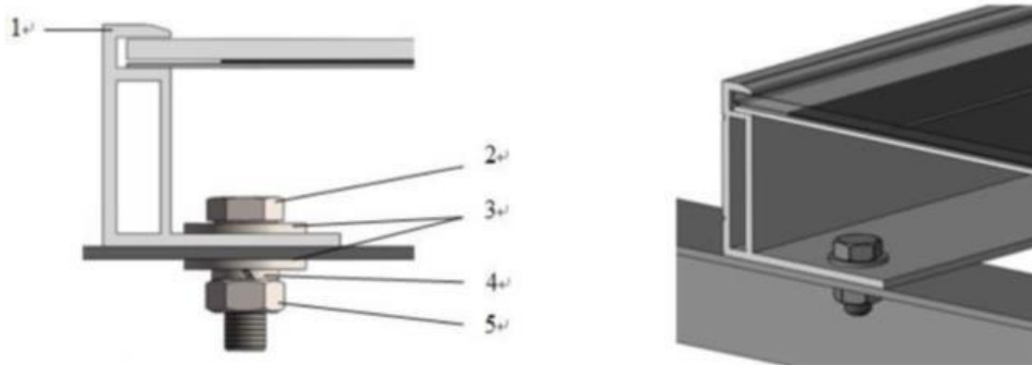
Fig.1 Backsheet-Glass module
